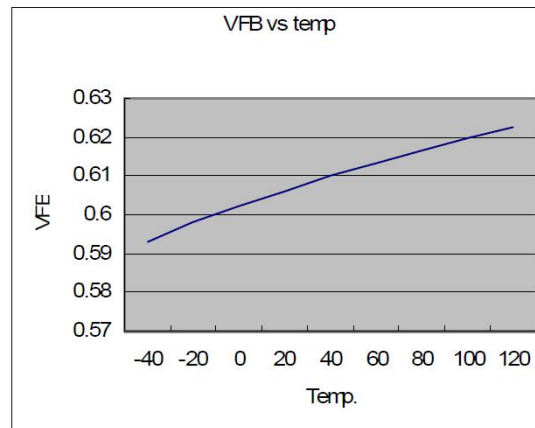
Feed back voltage vs. temp.
