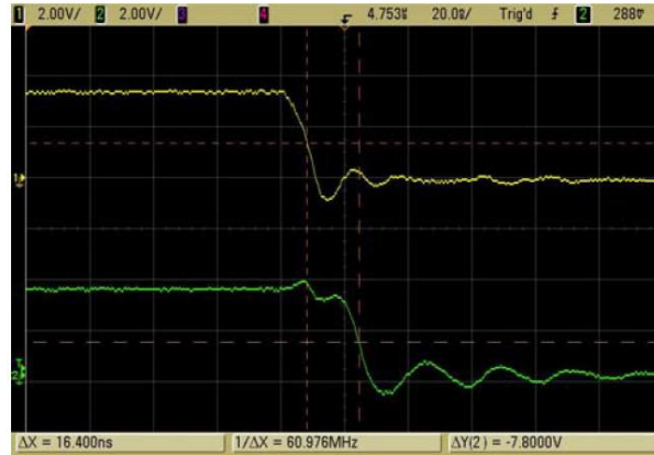
CKI to CKO delay time at falling edge(VCC=3.3V)
