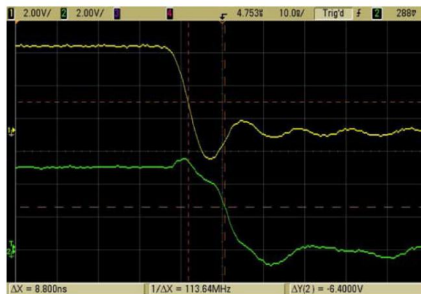
CKI to CKO delay time at falling edge(VCC=5V)
