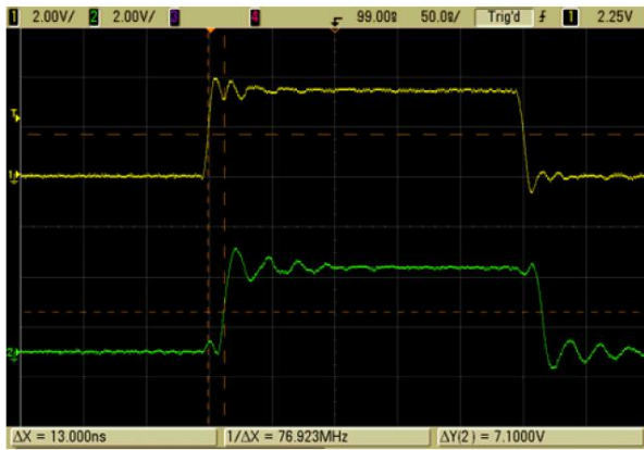
CKI to CKO delay time at rising edge(VCC=3.3V)
